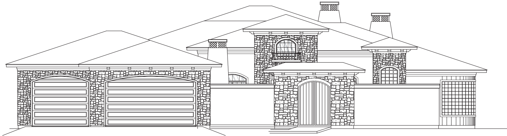
FRONT ELEVATION
